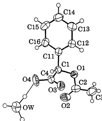
Fig. 1. A view of the asymmetric unit of H 3 O + .PhCH(OAc)CO 2 - showing the general conformation and our numbering scheme. The non-H atoms are shown with thermal ellipsoids drawn at the 50% probability level. For clarity the H atoms are drawn as small spheres of an arbitrary size. Only one of the two possible orientations for the methyl H atoms is shown.
