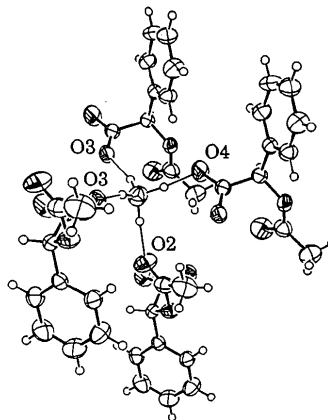
Fig. 2. A view showing the hydrogen-bonding environment around the oxonium cation with the three oxonium H atoms disordered over four sites.
